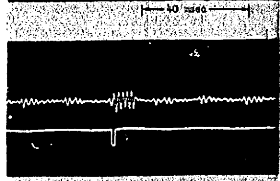
Fig. 3.67 Time comparison of second marks from WWV (top) and timer unit Shot No. 3 1000 km from ground zero
